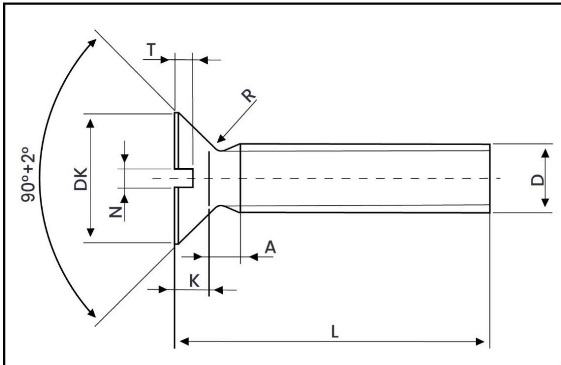
Weight Chart – DIN 963 Slotted Countersunk Flat Head Screw
