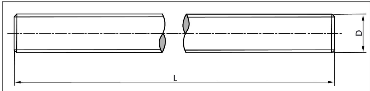
Weight Chart – DIN 976 Threaded Rod (Stud)
