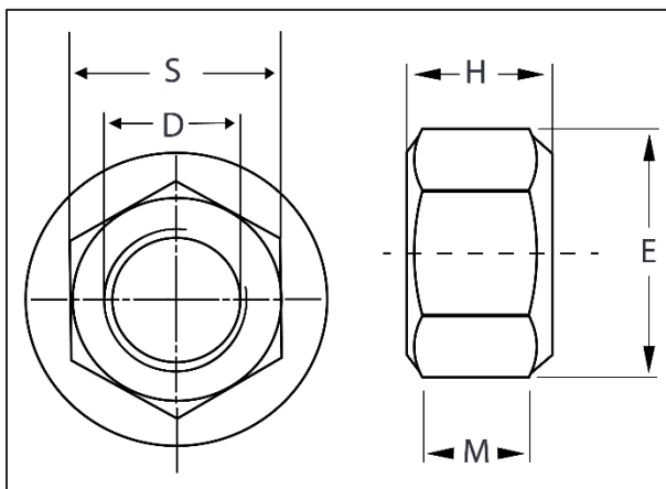
Weight Chart – DIN 982 Hex Lock Nut with Nylock Insert
