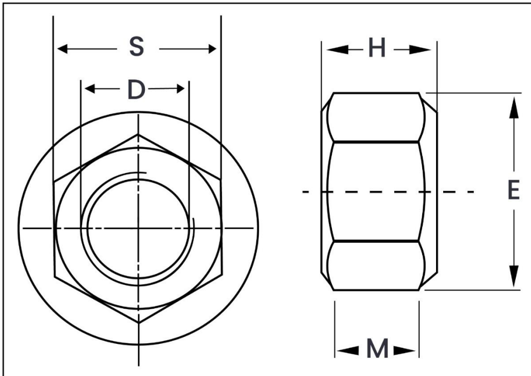
Weight Chart – DIN 985 Low Hex Lock Nut with Nylock Insert
